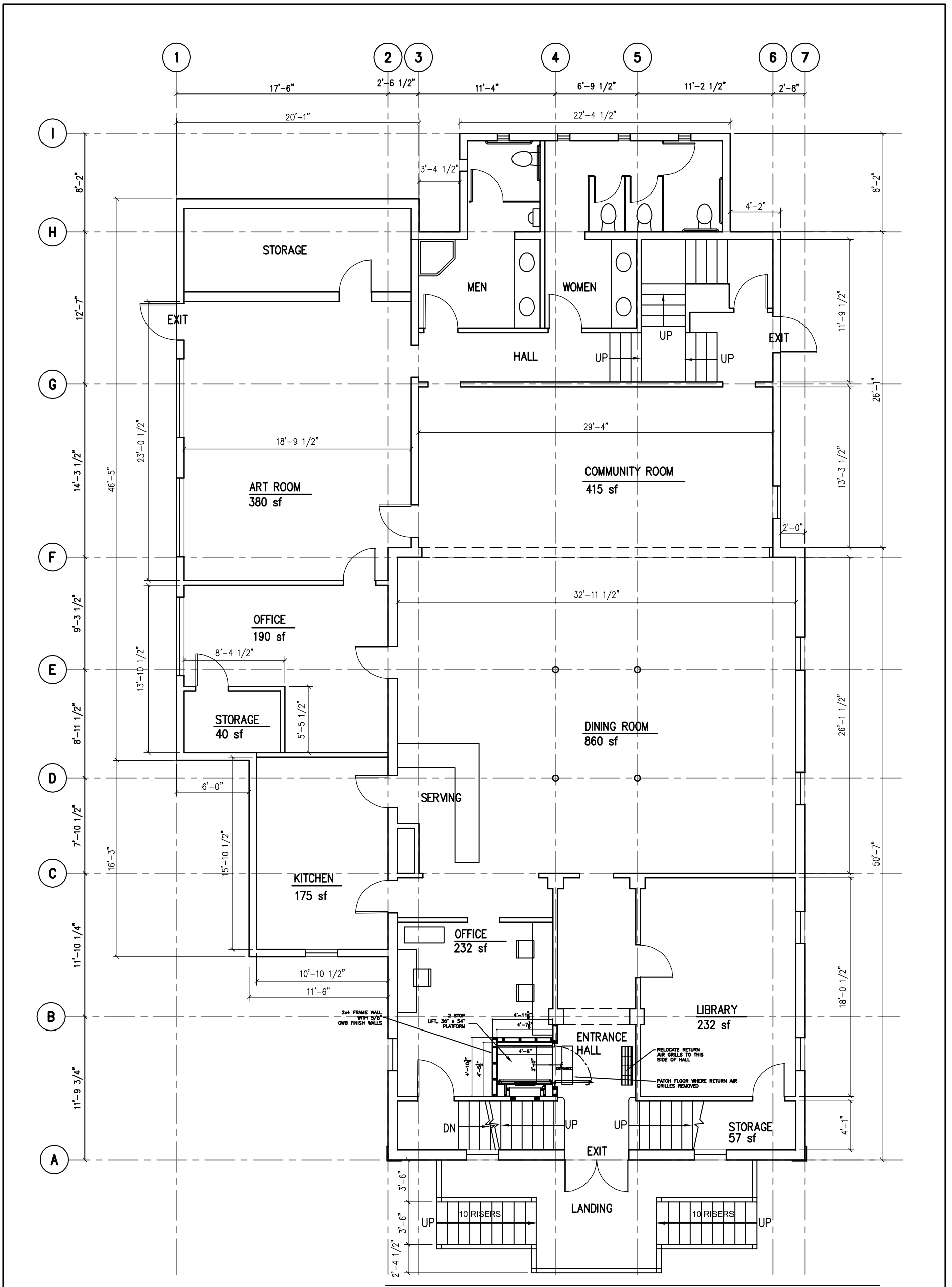
GROUND FLOOR
